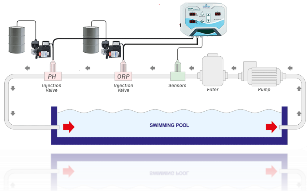
PH & ORP CHEMICAL CONTROLLER INSTALLATION DIAGRAM
